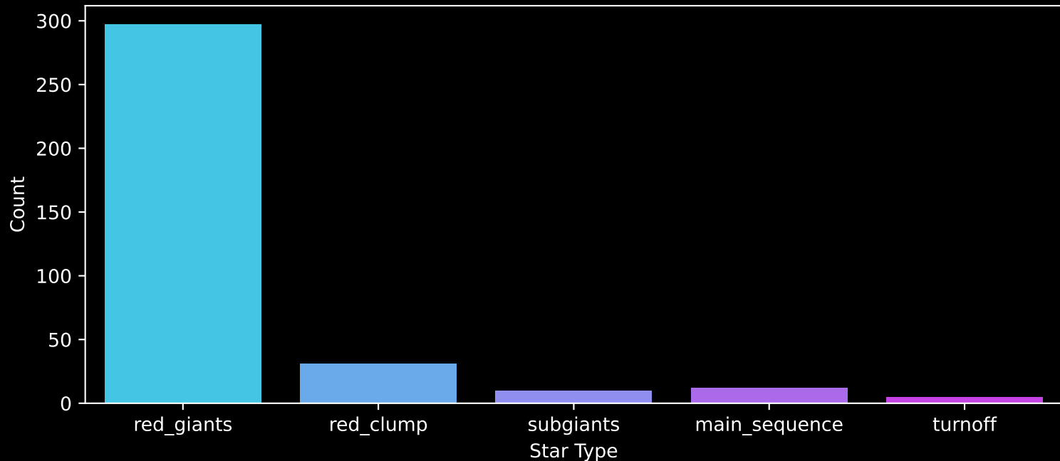
APOGEE DR17 Field: [015-12] Count plot of Star Type
