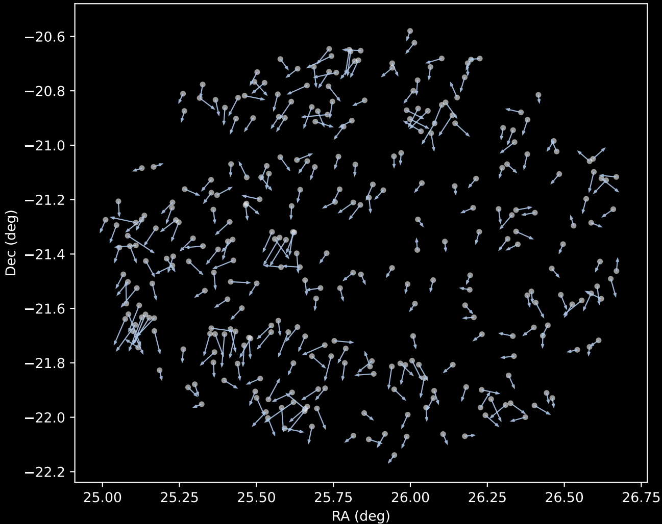
APOGEE DR17 Cluster 1 Proper Motion Vectors (n=312)
