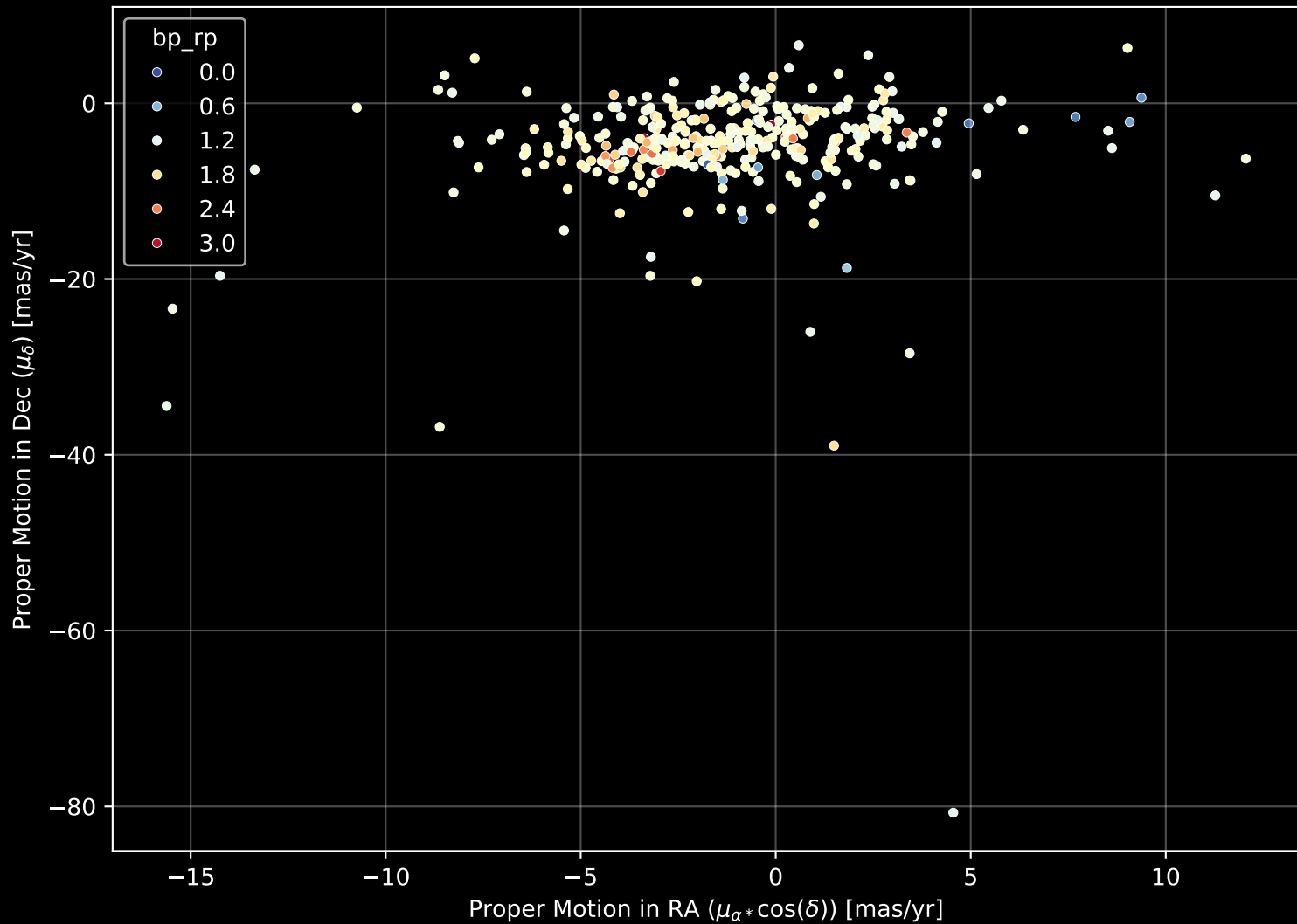
APOGEE DR17 Field: [015-12] Proper Motion Diagram (n= 355)
