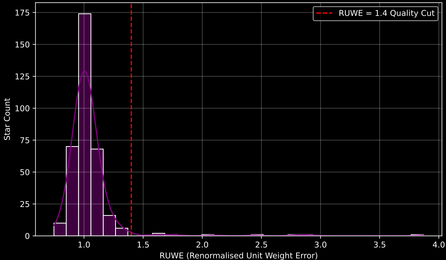
GAPOGEE DR17 Field [015-12] RUWE Distribution (n= 352)
