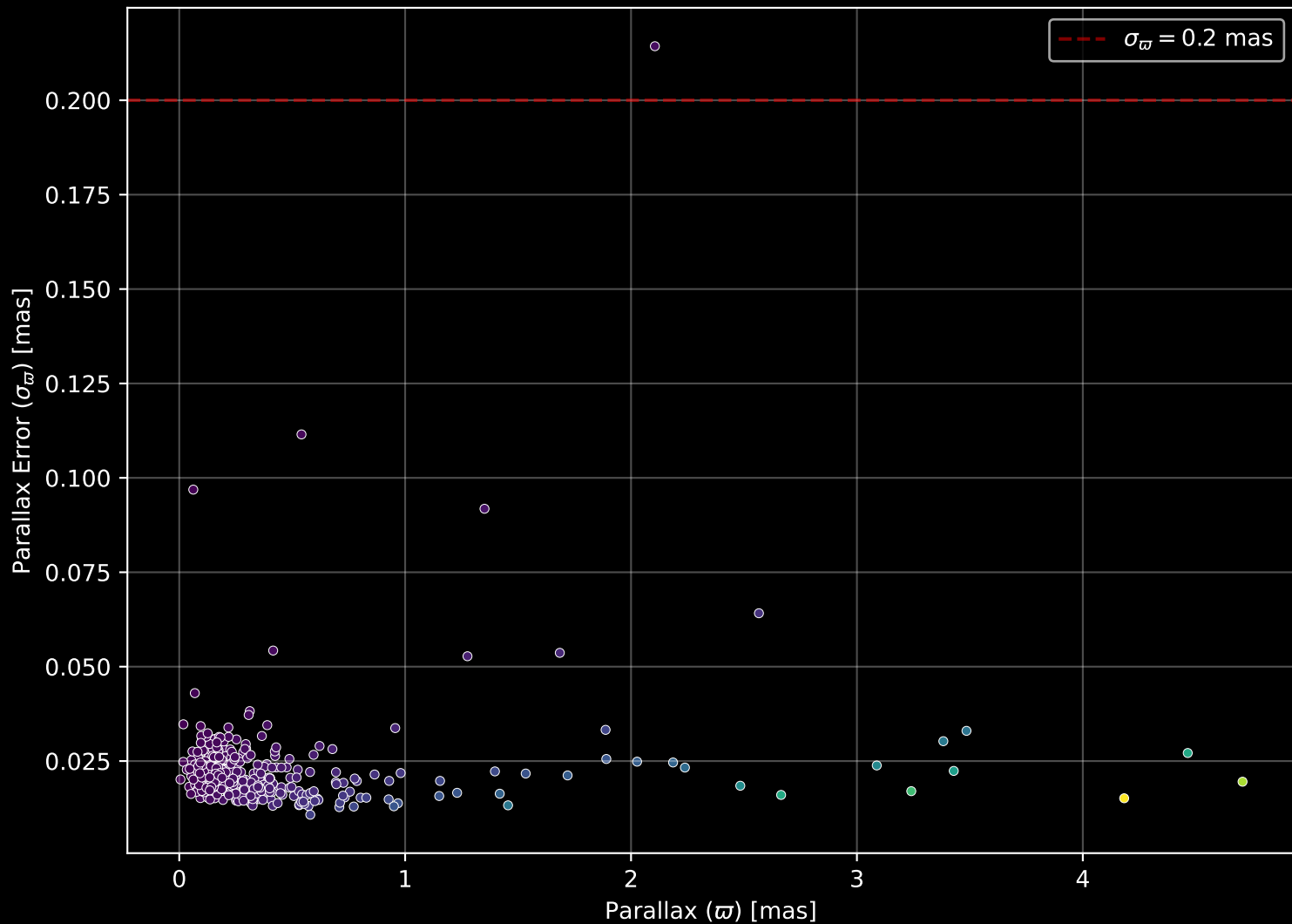
APOGEE DR17 Field: [015-12] Parallax Quality (n= 355)
