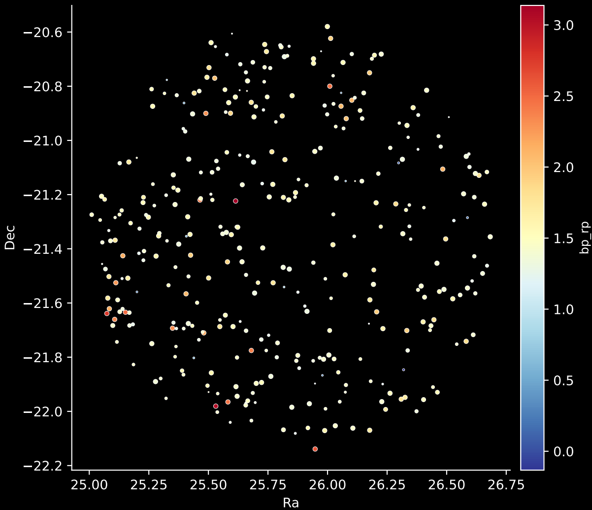
APOGEE DR17 Field: [015-12] Stars: 355
