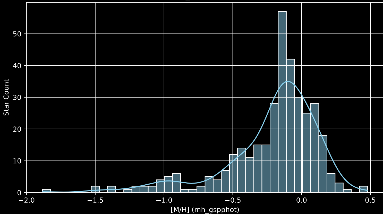
APOGEE DR17 Field: [015-12 [M/H] (mh_gspphot) (n= 354)
